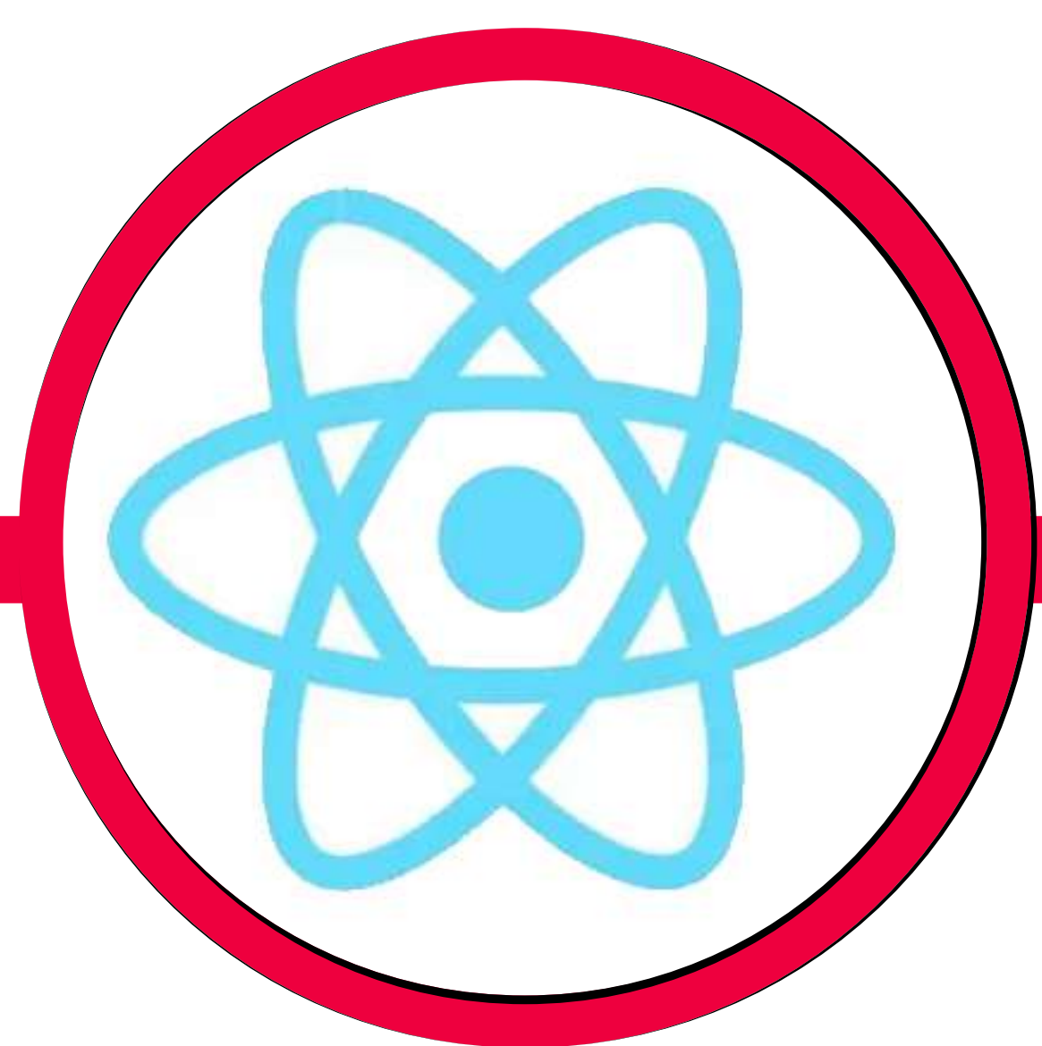
REACT JS
