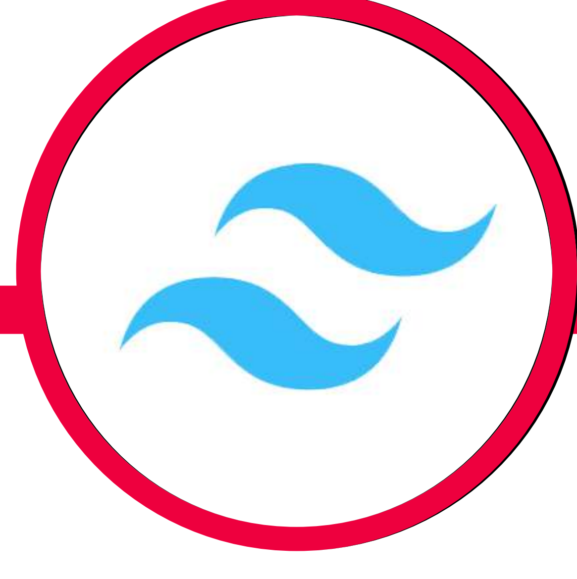
TAILWIND CSS
