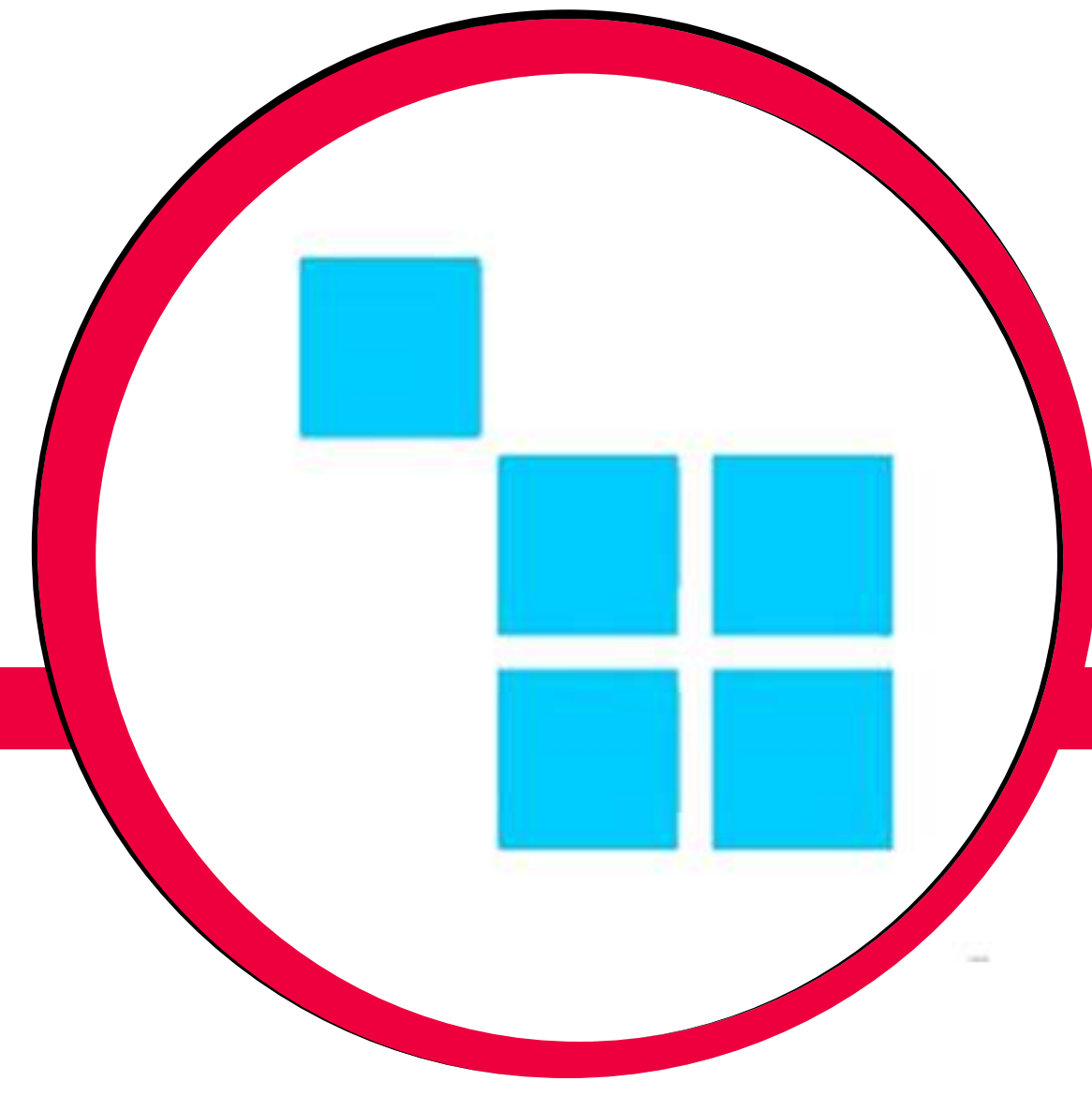
CS CART
