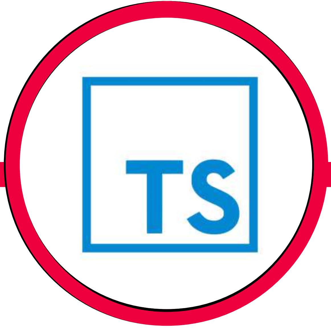
TYPESCRIPT
