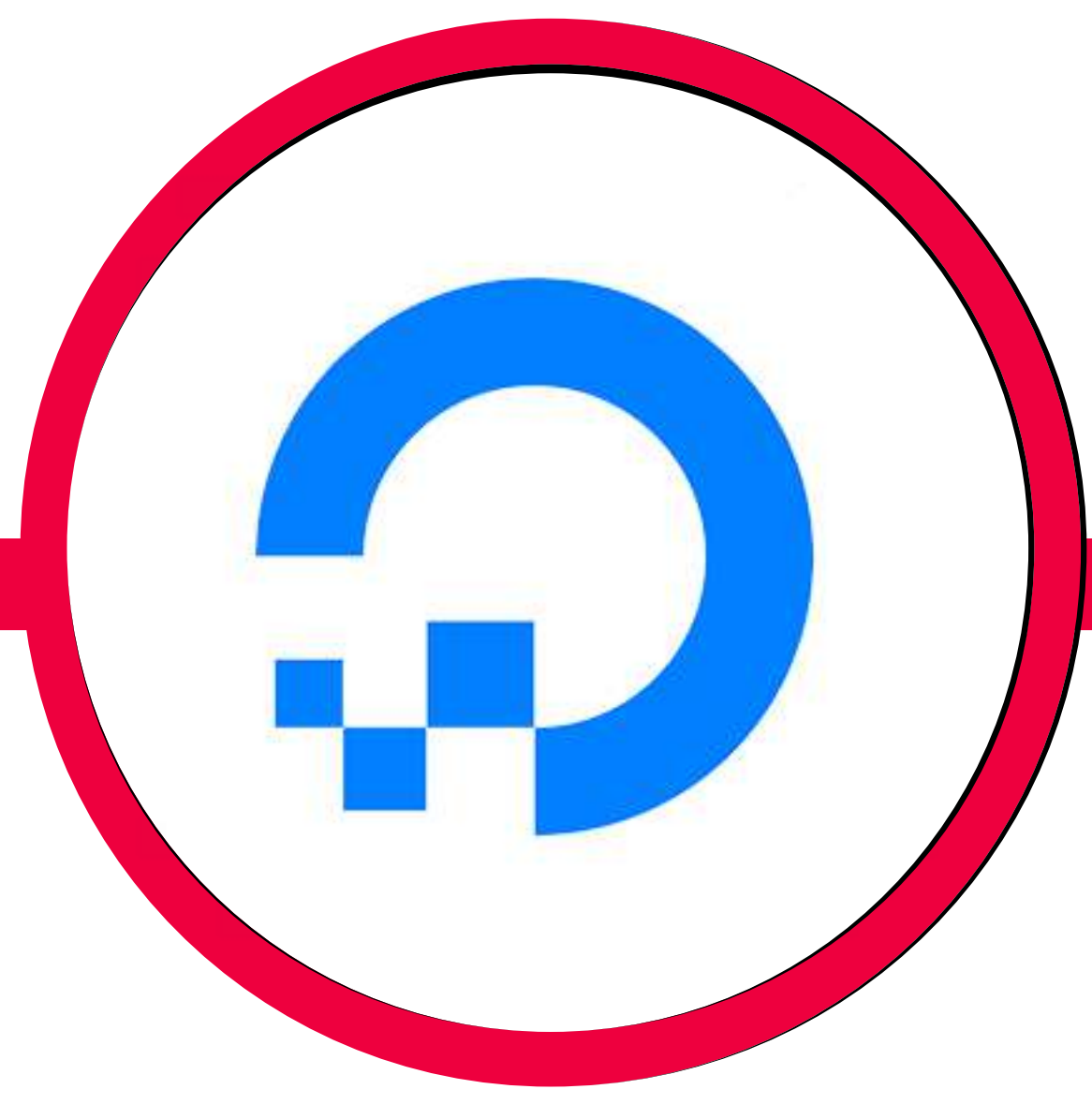
DIGITAL OCEAN
