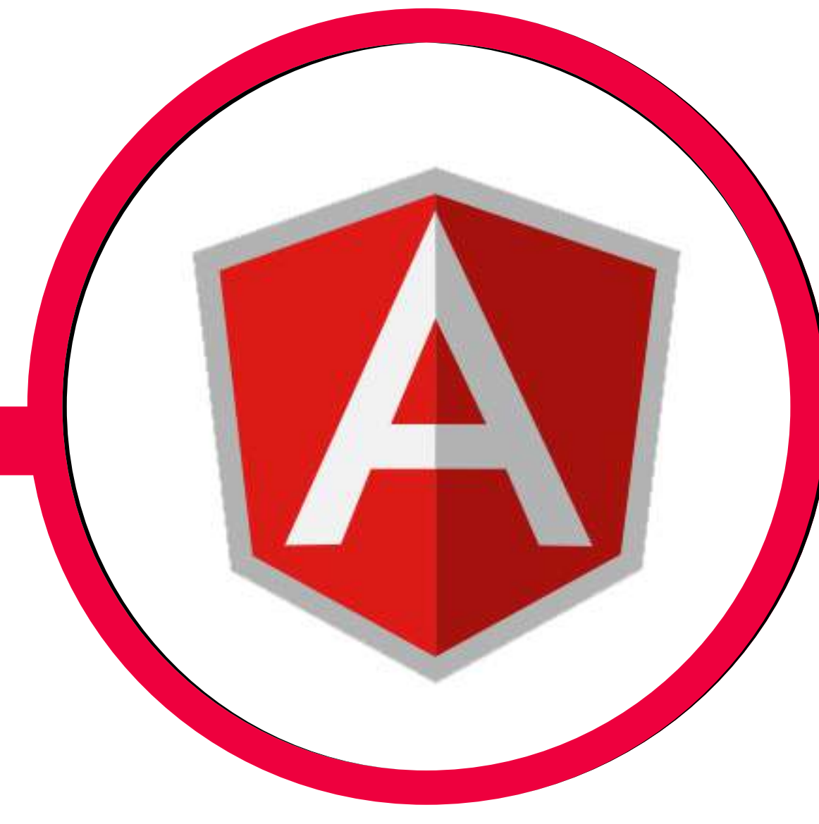
ANGULAR
