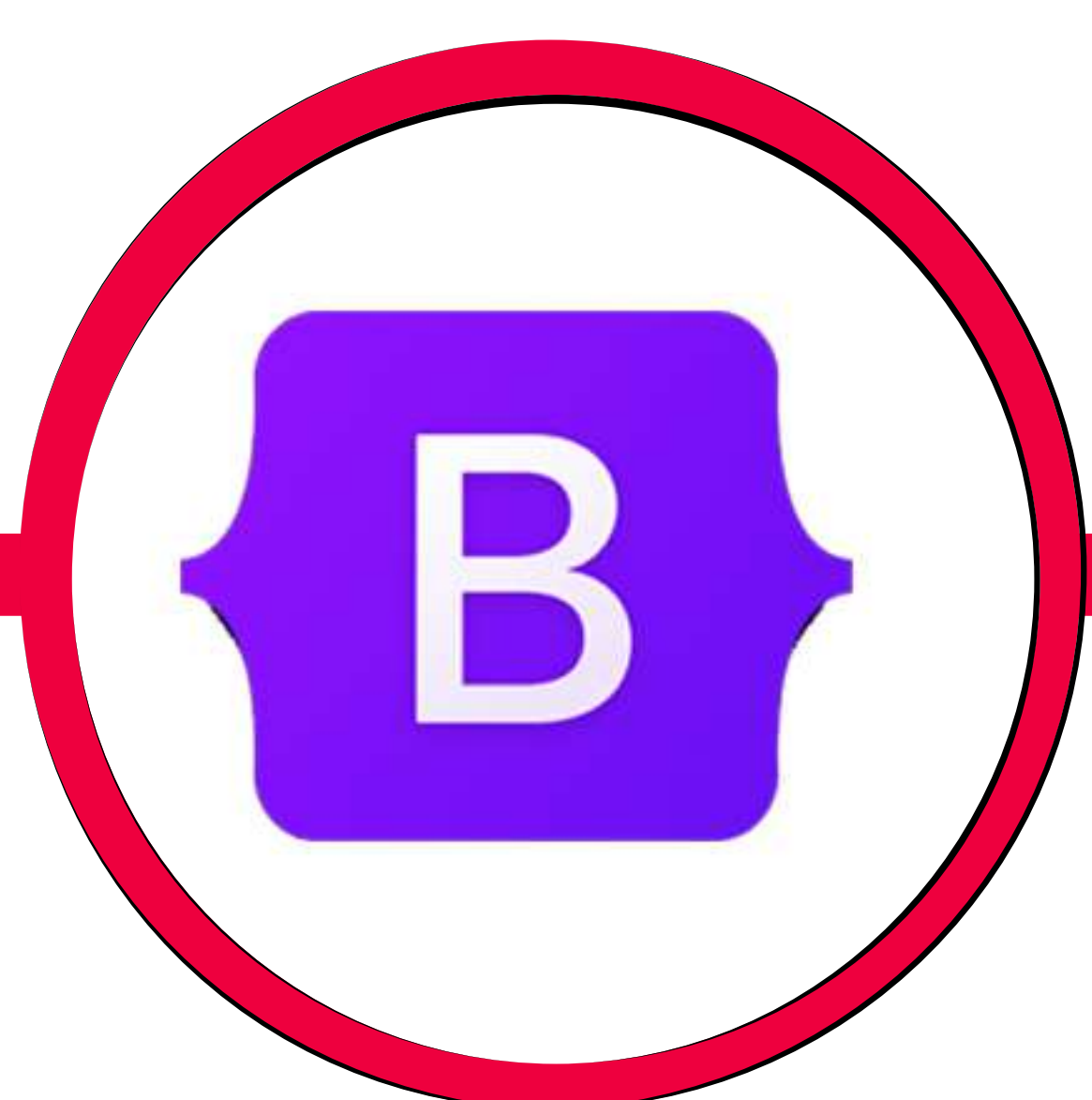
BOOTSTRAP
